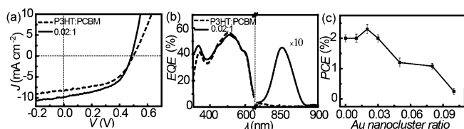
Figure 4. a) J – V curves of P3HT nanowire:PCBM and Au nanocluster loading in P3HT nanowire:PCBM (0.02:1 ratio). b) EQE spectra of nanohybrid solar cells with different Au nanocluster loading ratios. c) Power conversion efficiency of nanohybrid solar cells as a function of Au nanocluster loading ratios.
